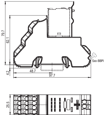
fig. 2. Dimension (mm)
