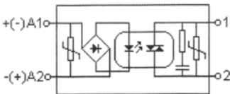
Fig. 1 CSS-AC diagram
